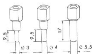
Punching Inserts
