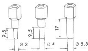
Punching Inserts
